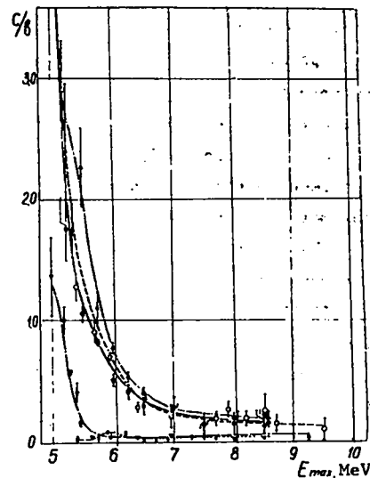
Fig. 2. Ratios of coefficients b/a and c/b as a function of E_{\max} : \times for ^{232}\text{Th} ; \nabla for ^{238}\text{U} ; \Delta , for ^{238}\text{Pu} ; \circ , for ^{240}\text{Pu} ; * , for ^{242}\text{Pu} .
