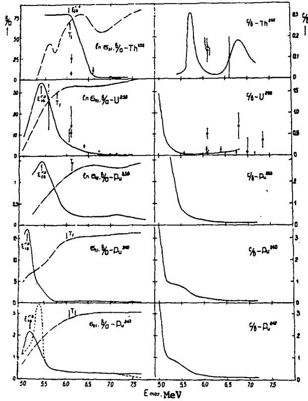
Fig. 6. Dependence of ratios b/a and c/b , obtained from curves of \sigma_1 in Fig. 3 (solid lines) and in \sigma_{Yf} in arbitrary units (dash line) on energy of \gamma -quanta, E . Points denote results of work of Ref. 3 (o), Ref. 18 (e), and Refs. 16 and 17 (□) for b/a and c/b . Dotted line shows b/a for variant treatment leading to irregularity in \sigma_a for ^{242}\text{Pu} (see Fig. 5).
